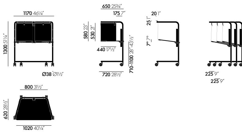
Scout Work Mobile
